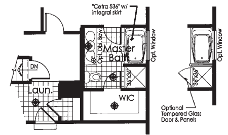
Glamour Master Bath Option
