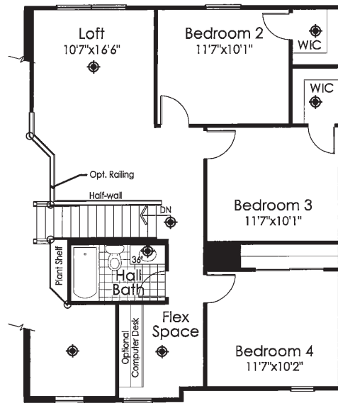
○ = Rounded Drywall Corners ◆ = LIGHT FIXTURE LOCATION Second Floor Plan
