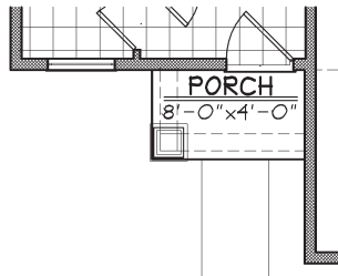
Partial Front Porch Plan
